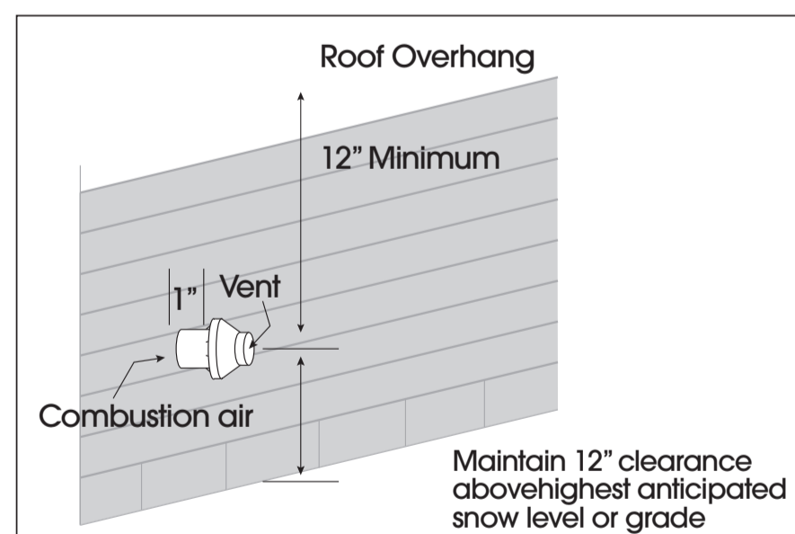
Figure 5-Sidewall Termination
