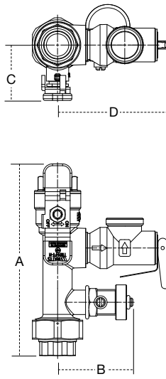
3/4" LFTWH-FT/FS-H-RV
