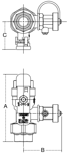
3/4" LFTWH-FT/FS-CN
